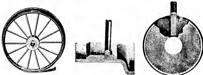
Figs. 5626-5628 THE CYRUS ROBERTS STEEL-TIRED WHEEL. Cast Hub, Steel Spokes and Felloe and Steel Flanged Tires. New tires may be shrunk on to center.
